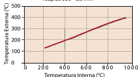
Gráfico de Performance Face Quente / Face Fria Teaplac 800 - 6,0 mm
